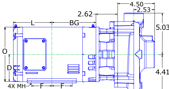
DRAWING DEPICTS JM145 3PHASE TEFC MOTOR ALL DIMENSIONS IN INCHES
